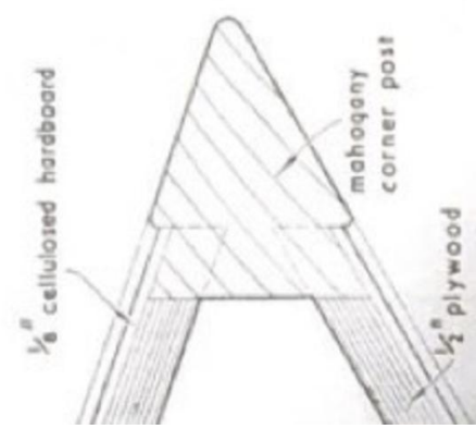
DETAIL AT A.
